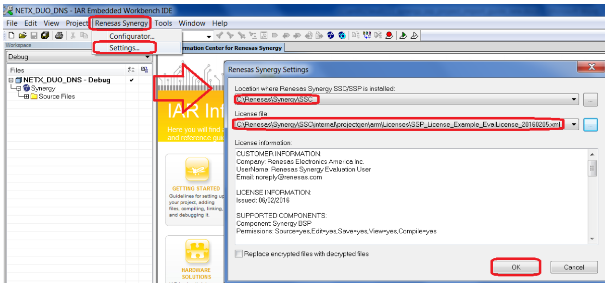
Figure 1.3 SSC/SSP settings
